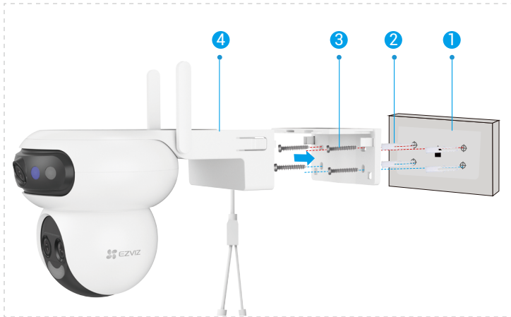
Fig. 2 Wall Mount
