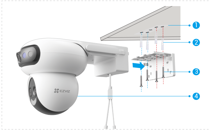
Fig. 1 Ceiling Mount
